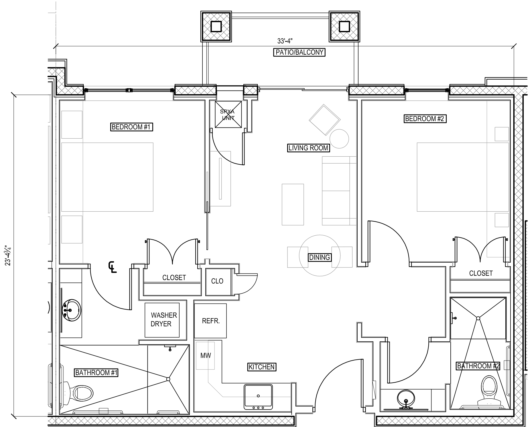
2 Bedroom Unit Floor Plan - ALF
